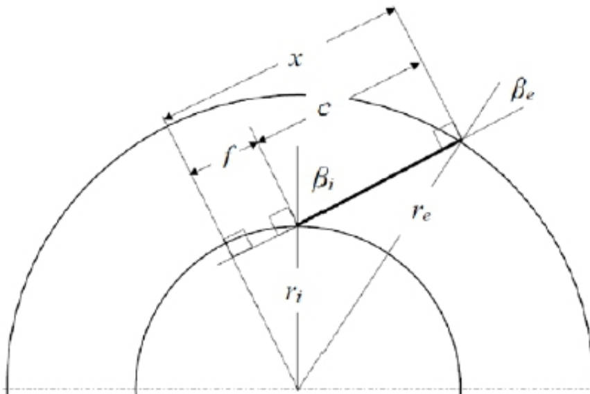
Figure 1 The geometry of impellers with straight, back-swept blades
